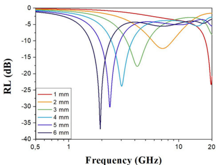
Reflection loss of FILAMAG-F TM 3D sheet of different thicknesses (simulated).
